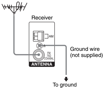
Outdoor FM antenna (aerial)
